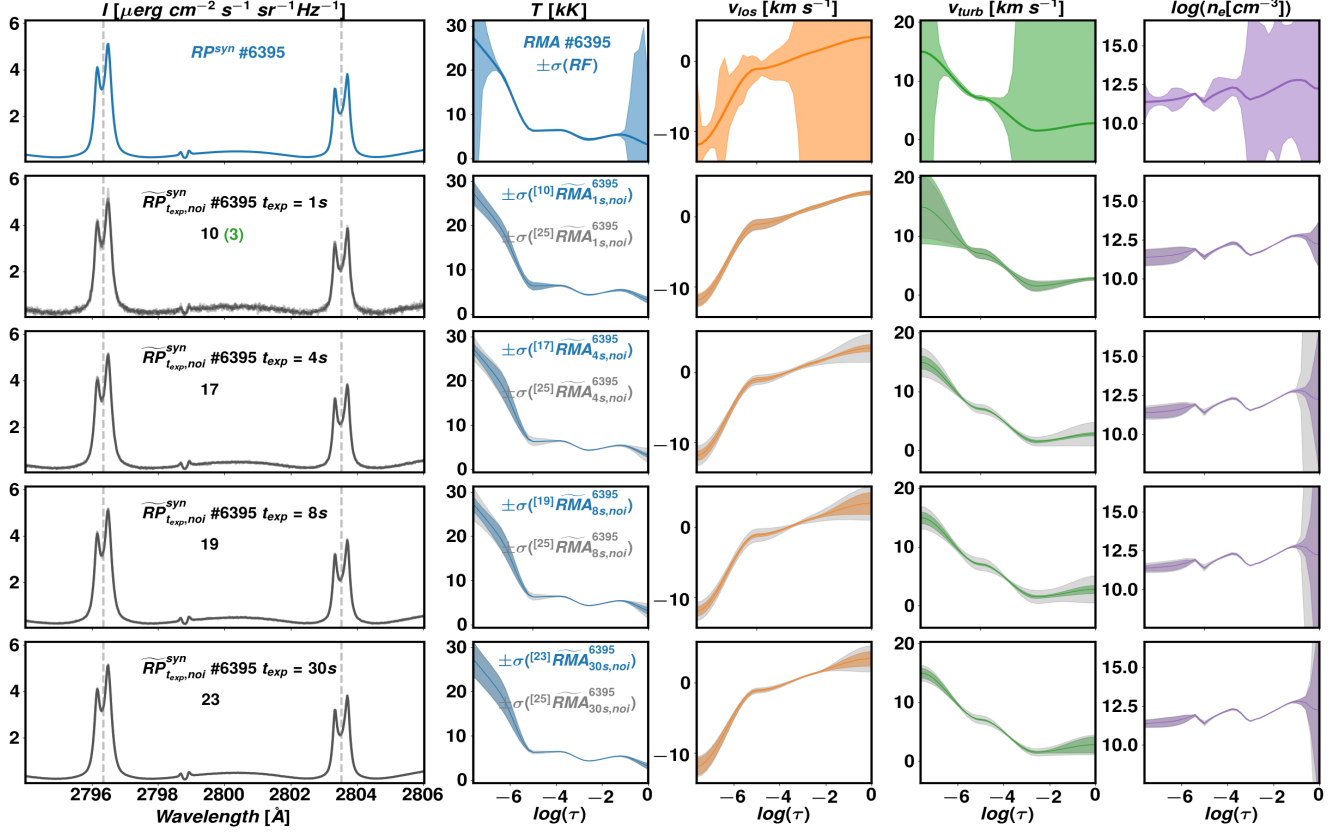
Figure 5. Same as Figure 4 for RP^{\text{syn}}\#6395 .
