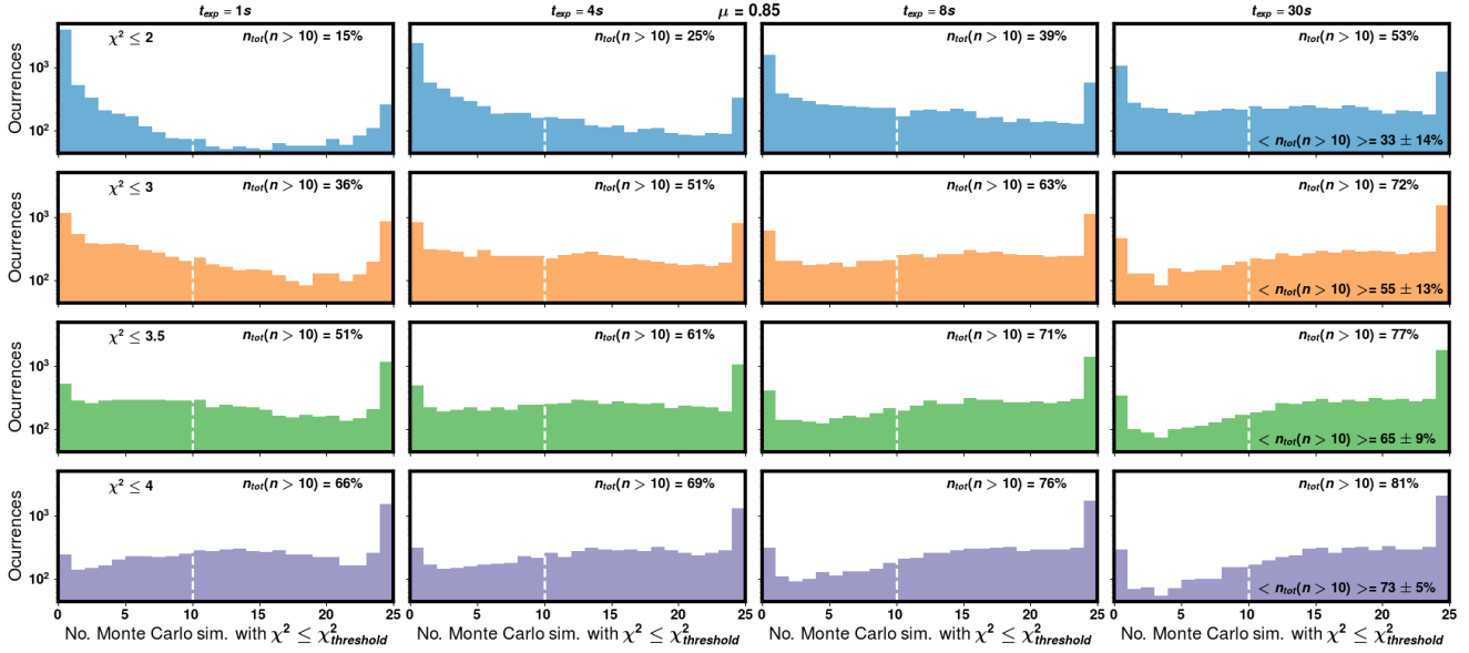
Figure 2. Histograms of number of Monte Carlo simulations (for all IRIS 2 entries with 0.8 \leq \mu < 0.9 ) for which \chi^2 \leq \chi^2_{\text{threshold}} , with different values of \chi^2_{\text{threshold}} in each row (indicated in upper left of each panel), and different exposure times in each column. Indicated in the top right of each panel is the fraction of cases for which there are at least 10 Monte Carlo simulations with a goodness of fit better than \chi \leq \chi^2_{\text{threshold}} .
