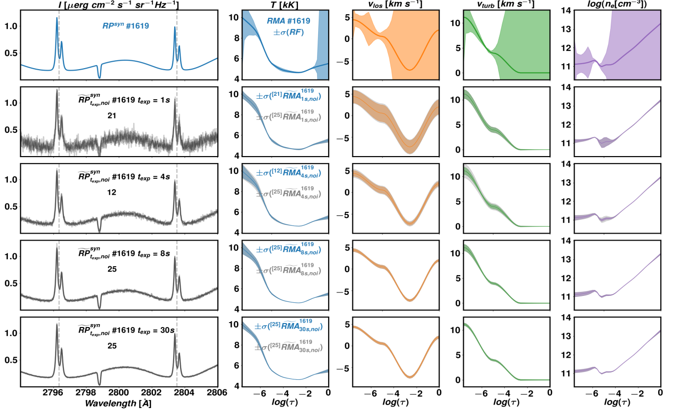
Figure 4. The first column shows the RP^{\text{syn}}\#1619 in blue, and in black its \widetilde{RP}_{t_{\text{exp}},\text{noi}}^{\text{syn}} for t_{\text{exp}} = 1, 4, 8, and 30\text{s} . The corresponding RMA for T, v_{\text{los}}, v_{\text{turb}}, and n_e and their uncertainties are shown from the second to the fifth column respectively. In the first row, the uncertainty is obtained from the response functions, while the ones from the second to the fifth rows are obtained by using N Monte Carlo experiments as shown in ^{[N]}\widetilde{RMA}_{t_{\text{exp}},\text{noi}}^{\text{syn}} , for t_{\text{exp}} = 1, 4, 8, and 30\text{s} respectively.
