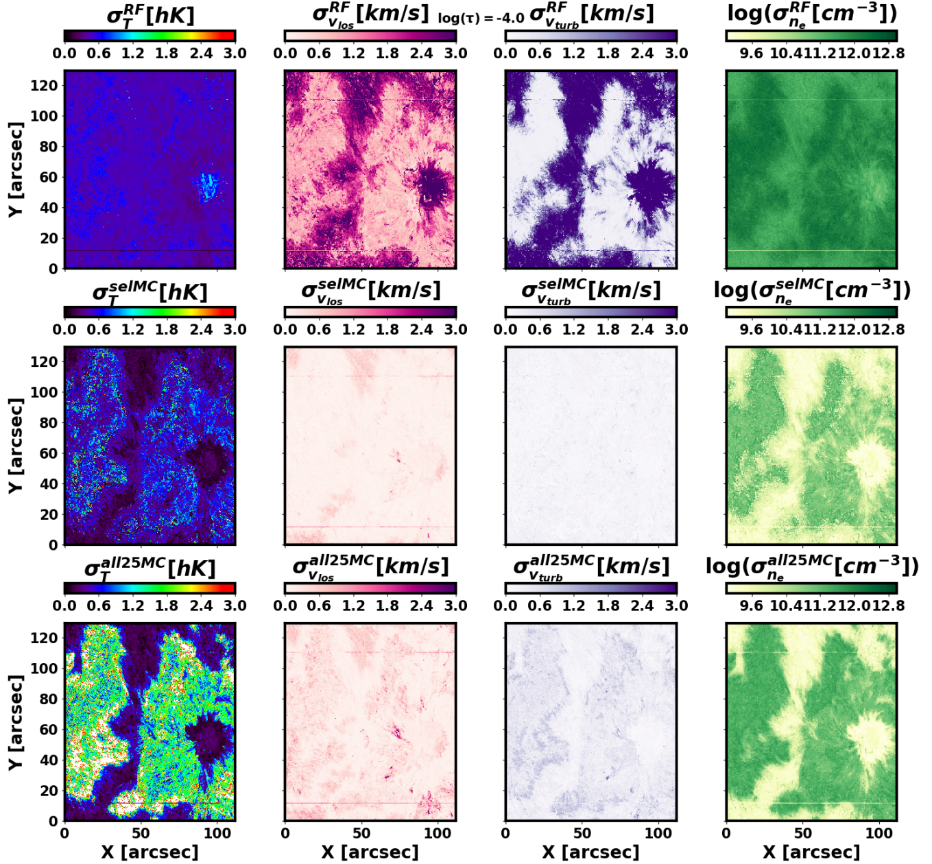
Figure 6. The uncertainties for the T , v_{los} , v_{turb} , and n_e at \log(\tau) = -4 when considering the RFs (top row), the selective Monte Carlo approach (middle row), or all the 25 Monte Carlo experiments (bottom row).
