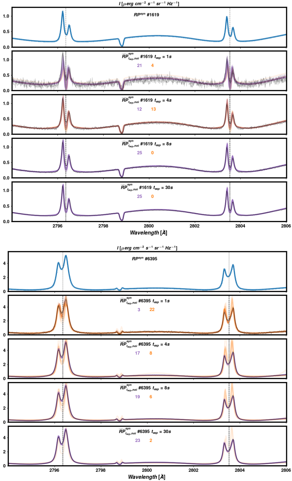
Figure 1. Top panel: The RP^{syn} #1619 is shown in the first row. The four following rows show their corresponding \widetilde{RP}_{t_{exp},noi}^{syn} (in black) for t_{exp} = 1, 4, 8 and 30 s, and the "good" and "bad" MC fits in violet and orange respectively (the colored numbers indicate the number of "good" and "bad" MC fits). Bottom panel: the same for RP^{syn} #6395.
